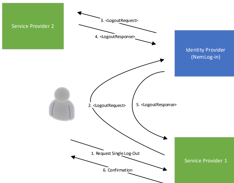
FIGURE 5: SINGLE LOG-OUT
